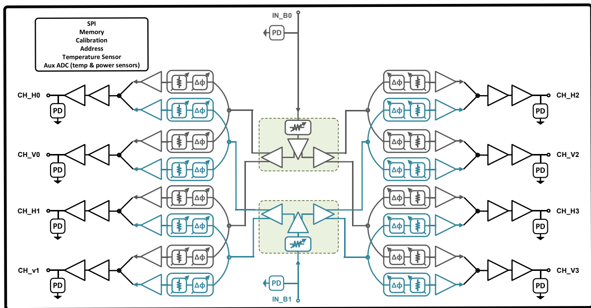
Figure 1.1.1: Stampede2731 Block Diagram
