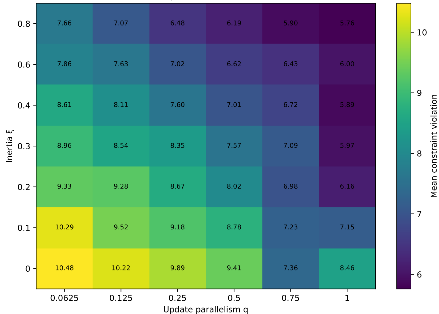
Full-resident TSP: permutation-constraint violation
