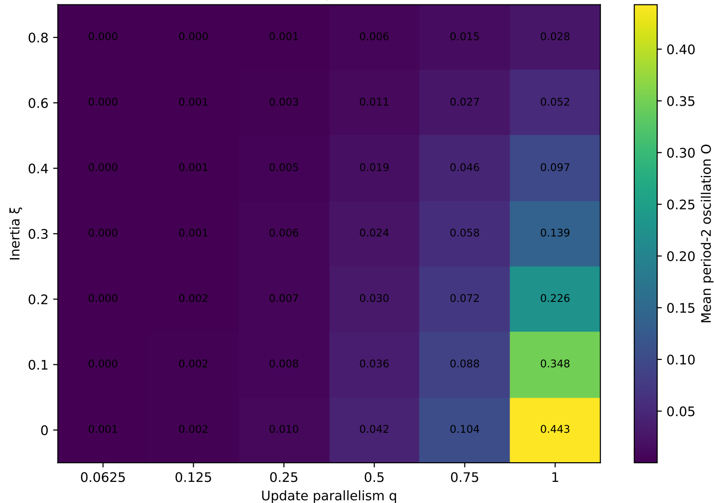
Full-resident TSP: period-2 oscillation
