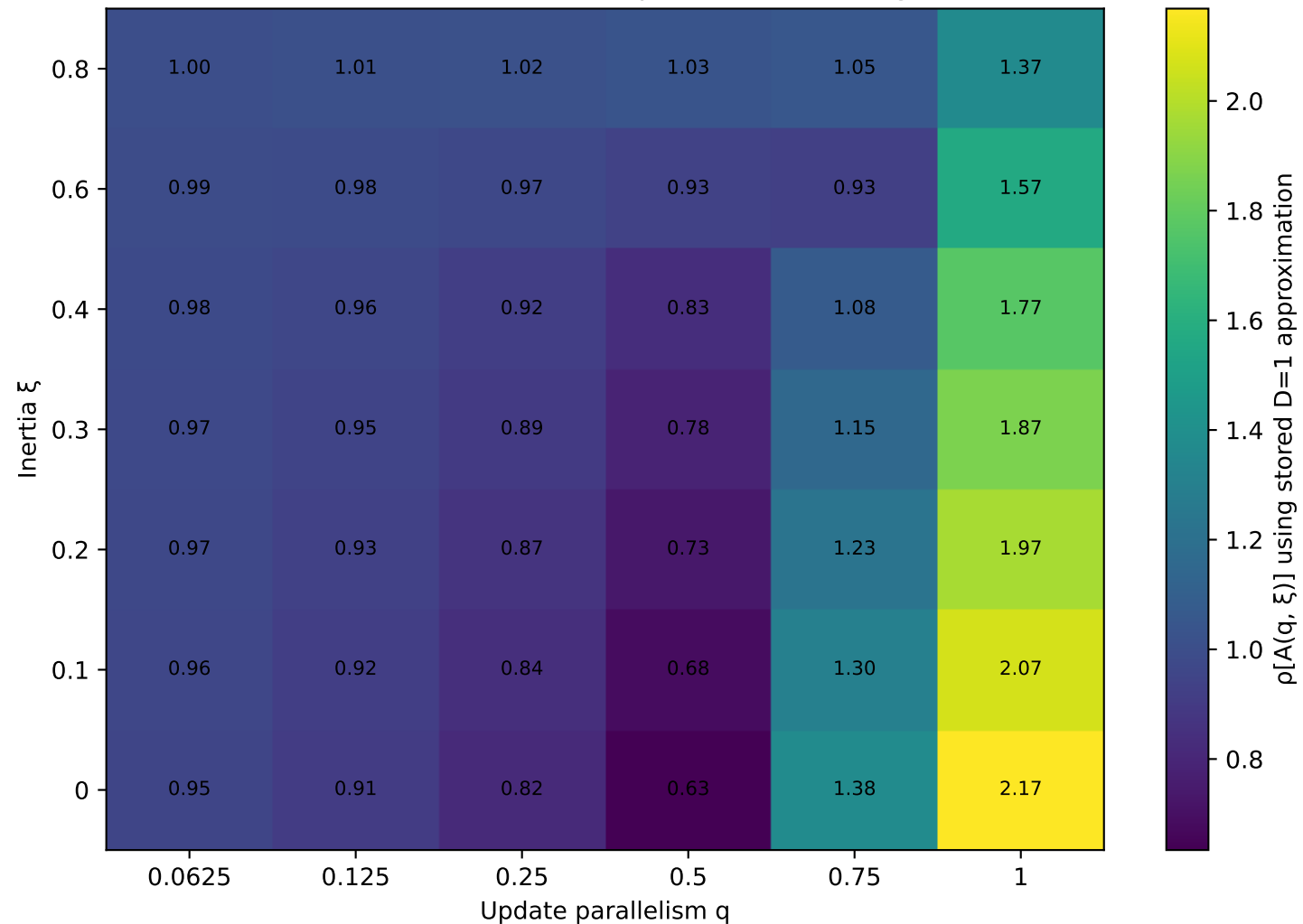
Full-resident TSP: linearized spectral-radius diagnostic
