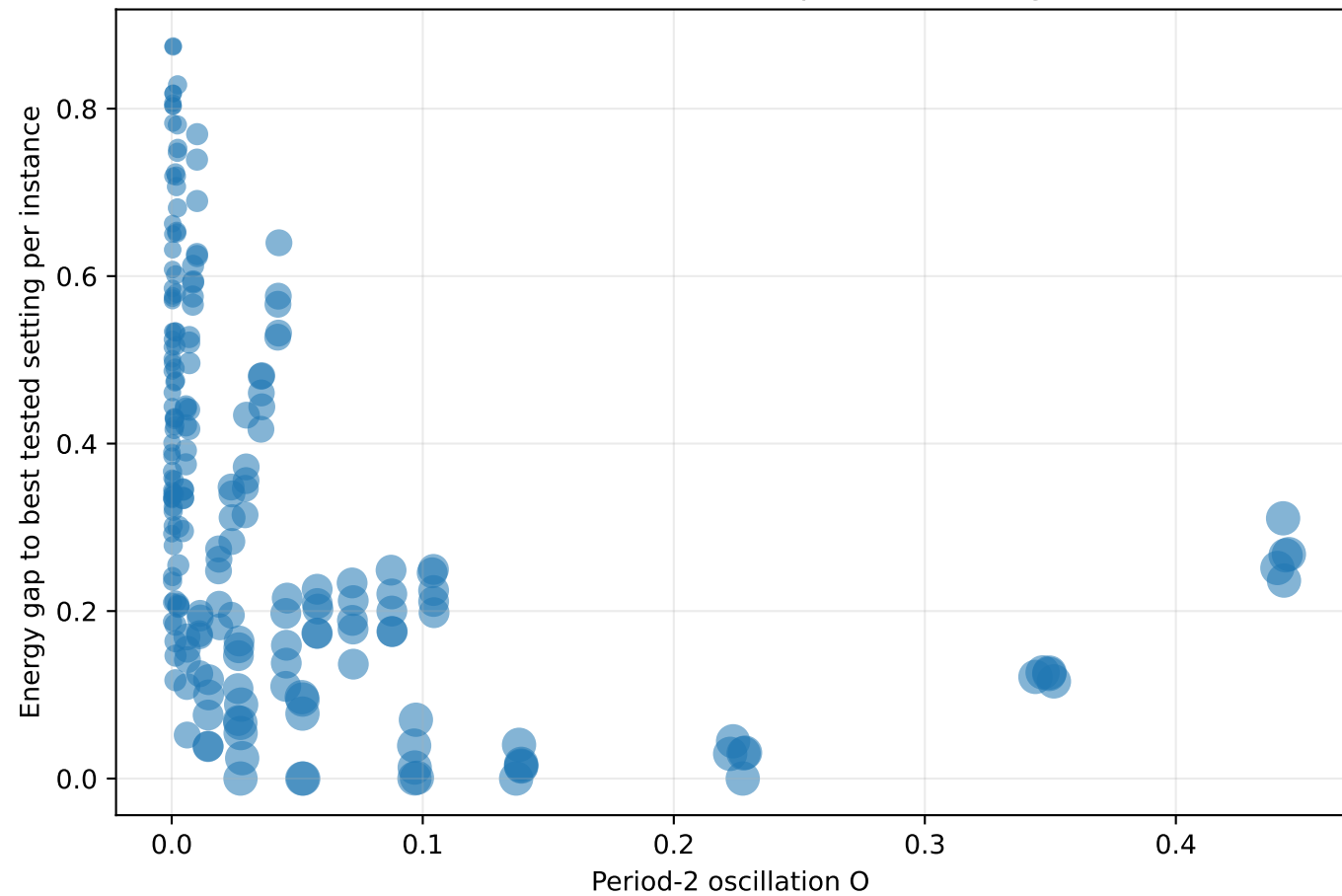
Full-resident TSP: oscillation vs optimization degradation
