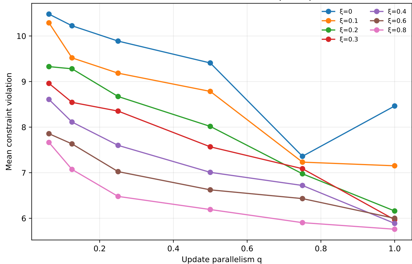
Full-resident TSP: constraint violation vs update parallelism
