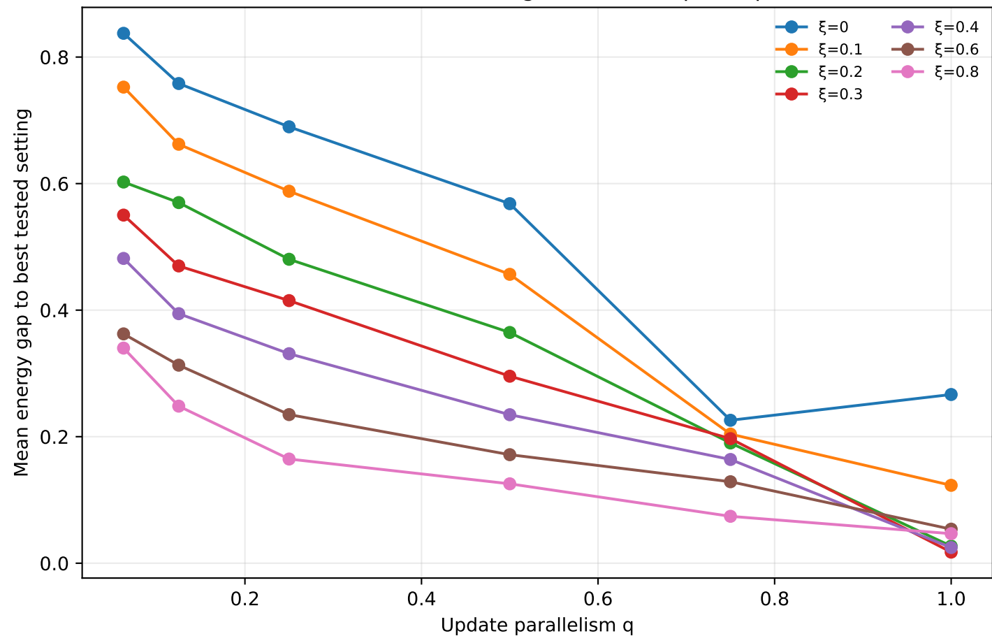
Full-resident TSP: solution degradation vs update parallelism
