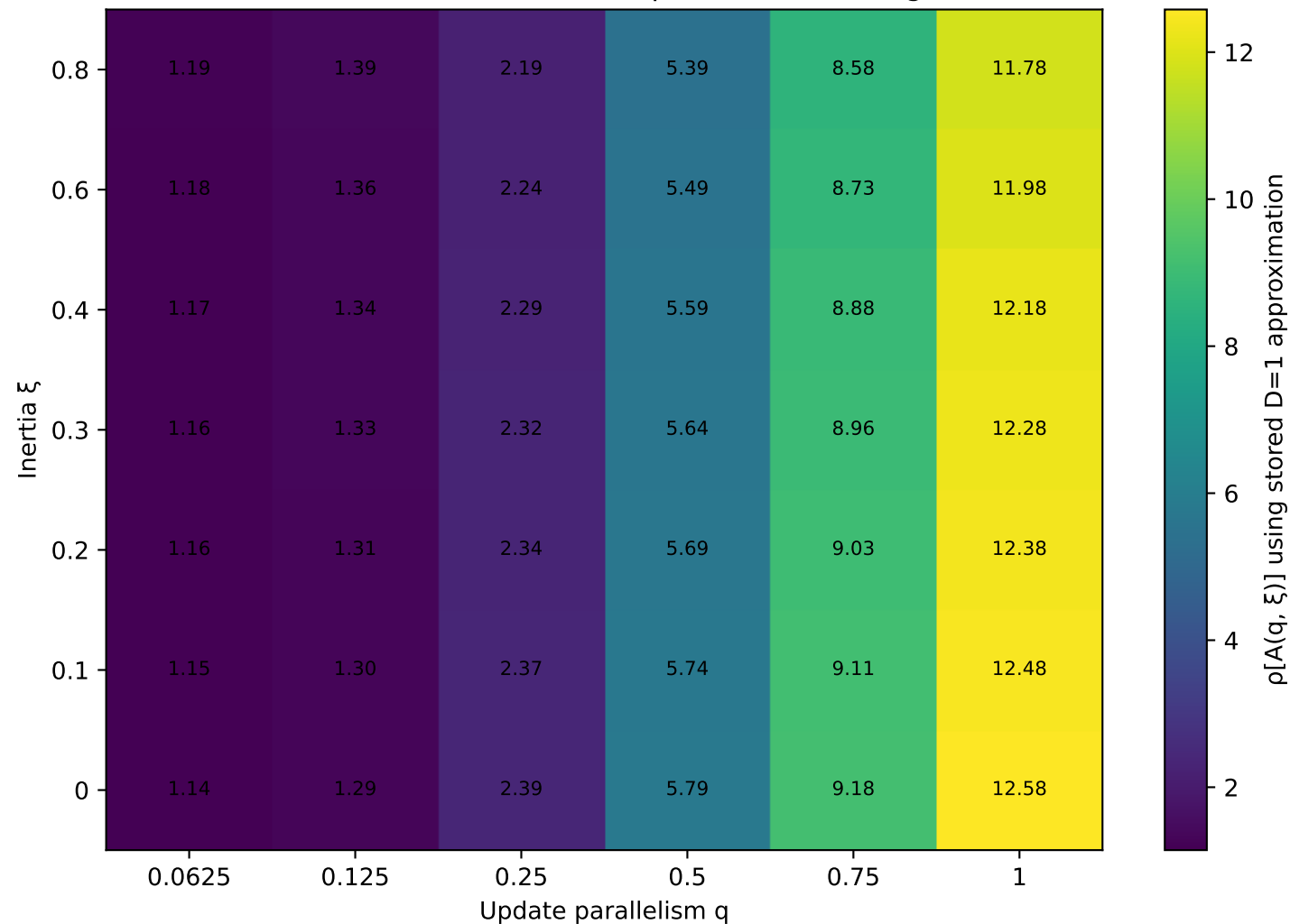
Dense ER Max-Cut: linearized spectral-radius diagnostic
