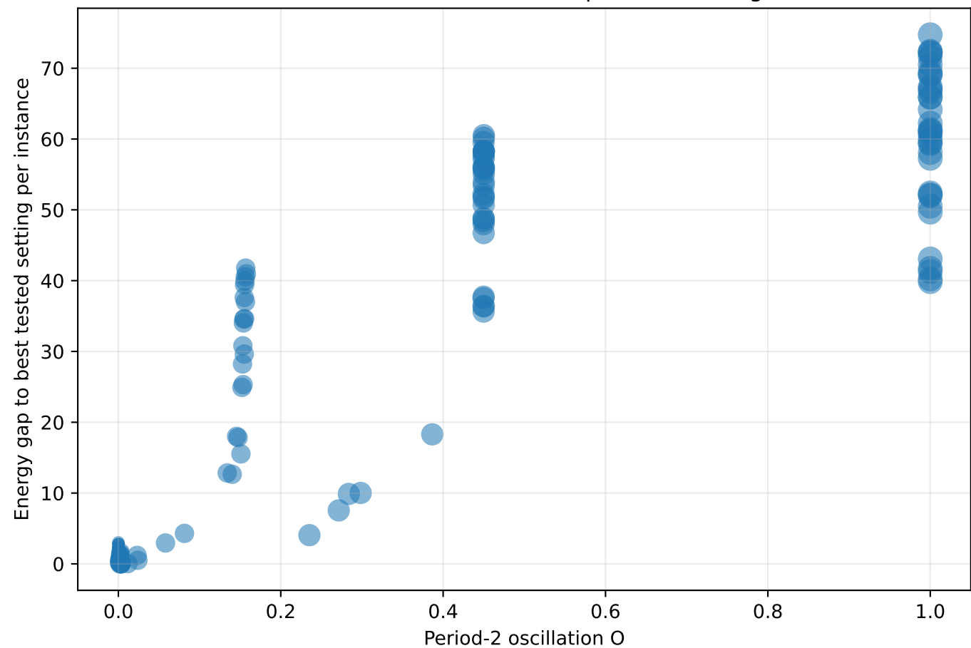
Dense ER Max-Cut: oscillation vs optimization degradation
