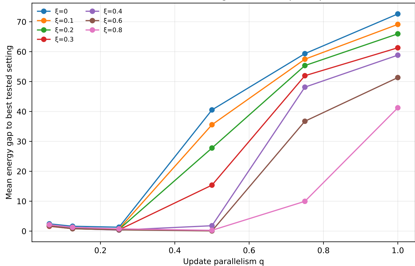
Dense ER Max-Cut: solution degradation vs update parallelism
