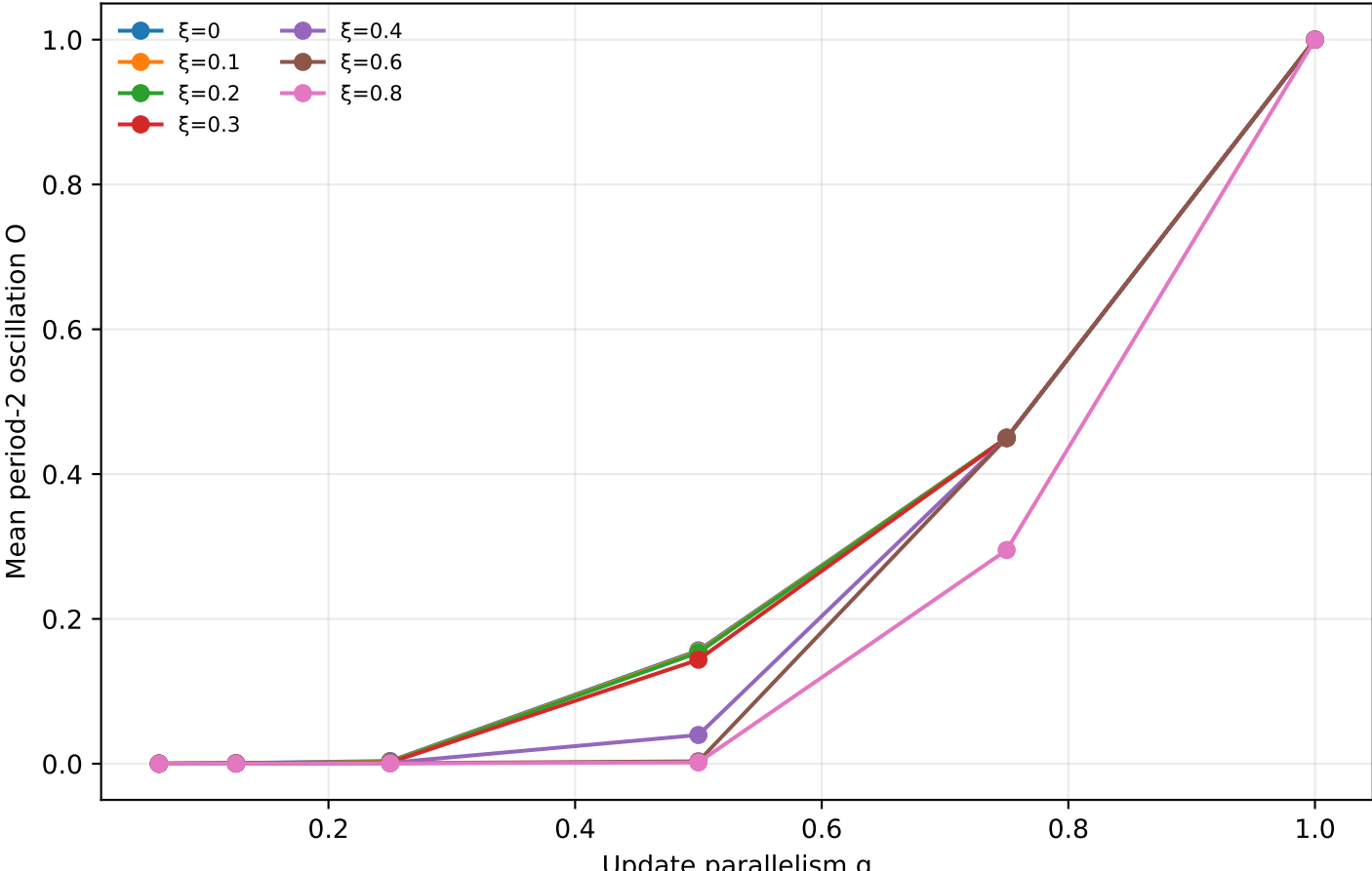
Dense ER Max-Cut: oscillation vs update parallelism
