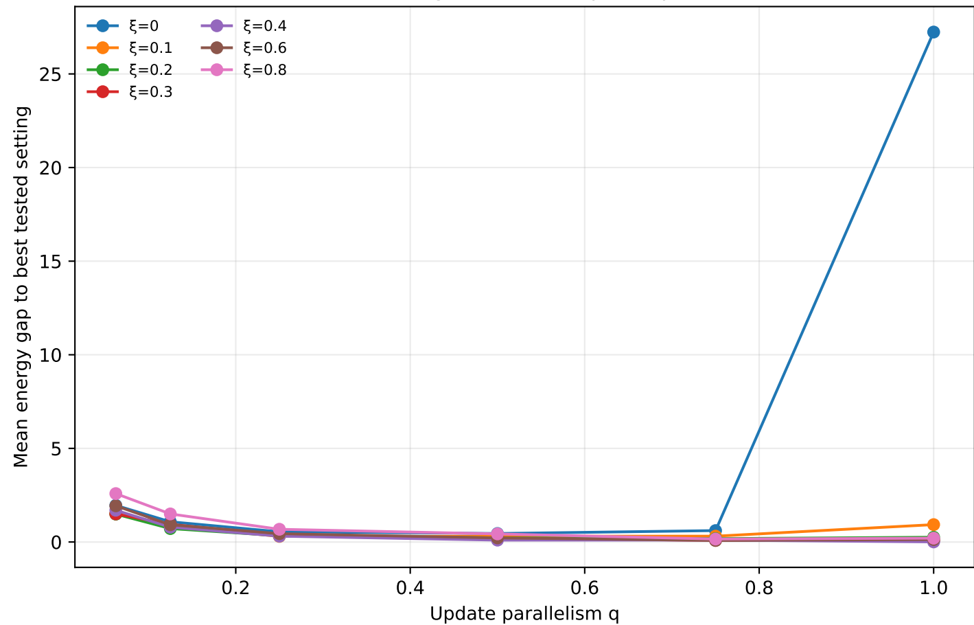
SK: solution degradation vs update parallelism
