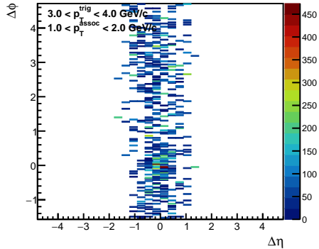
Multi-jet Events
