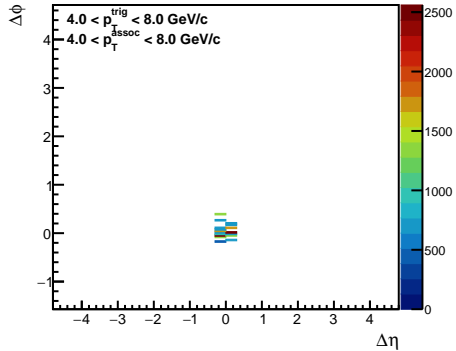
Single-jet Events
