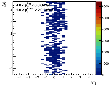
Dijet Events
