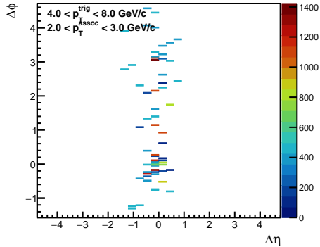
Multi-jet Events
