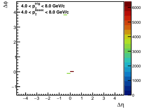
Multi-jet Events
