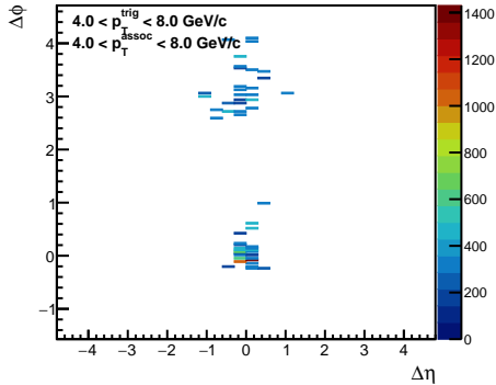
Dijet Events
