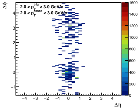
Dijet Events
