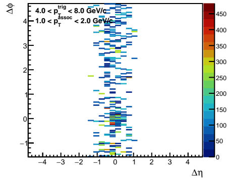
Multi-jet Events
