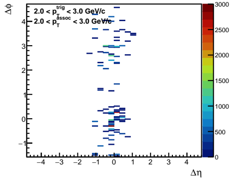
Multi-jet Events
