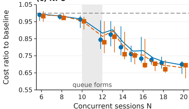
(c) NPU
