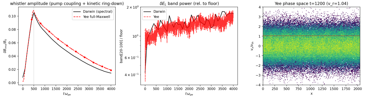
Figure 2: Darwin (spectral) vs Yee (full-Maxwell) branch on the same input deck (An et al. Sim 3): whistler amplitude history (left), secondary electrostatic band power over the noise floor (middle), and Yee-branch phase space at t = 1200 \omega_{pe}^{-1} (right).
