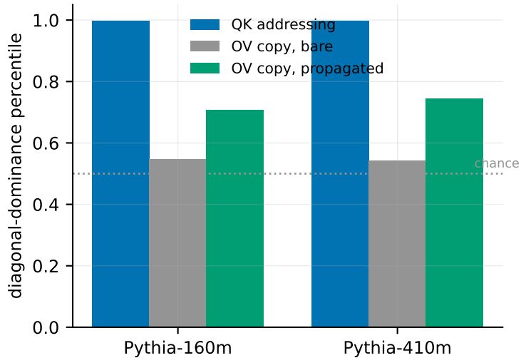
(a) real LM: addressing = associative memory
