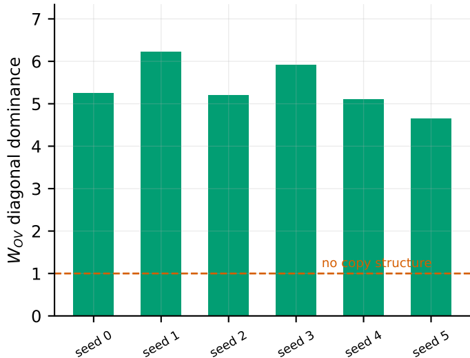
(b) toy: OV is a copy operator (copy fidelity = 1.0)
