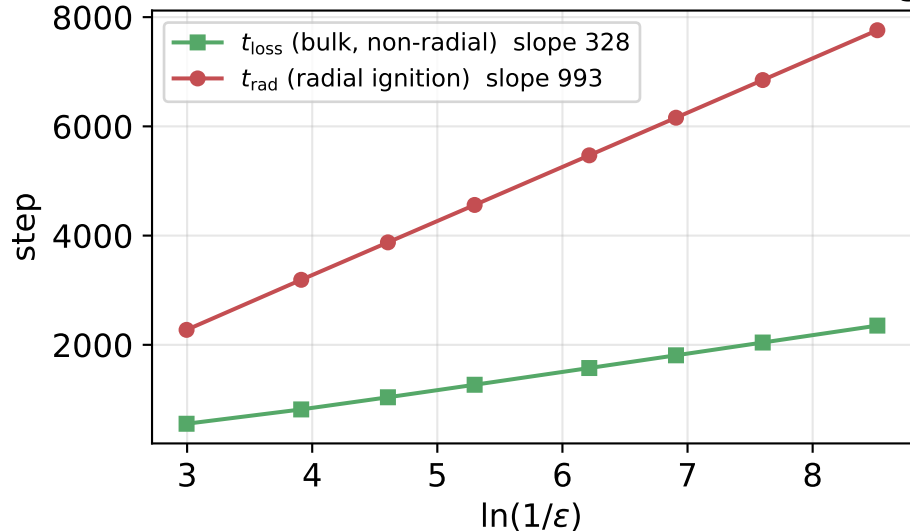
(b) Radial mode has the slower \varepsilon -scaling
