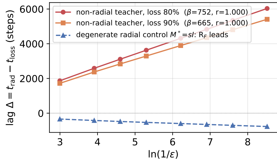
(a) Lag grows as \beta \ln(1/\varepsilon) , \beta > 0
