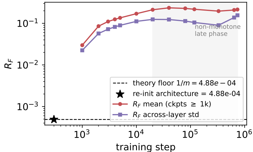
(a) OLMo-1B: floor (re-init) + post-ignition differentiation (b) Differentiation through the bulk; non-monotone late phase
