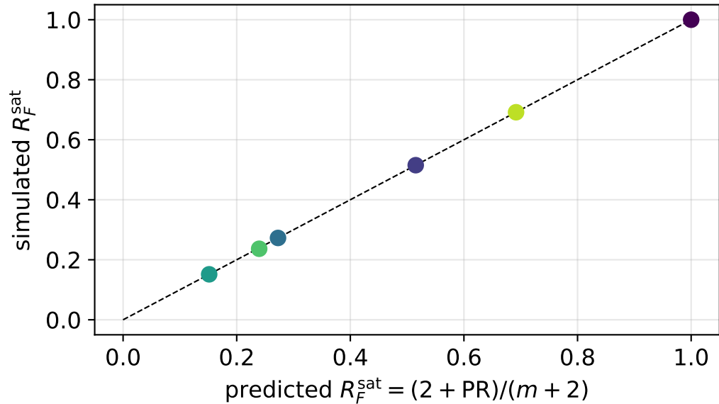
(b) Saturation = spectral participation ratio
