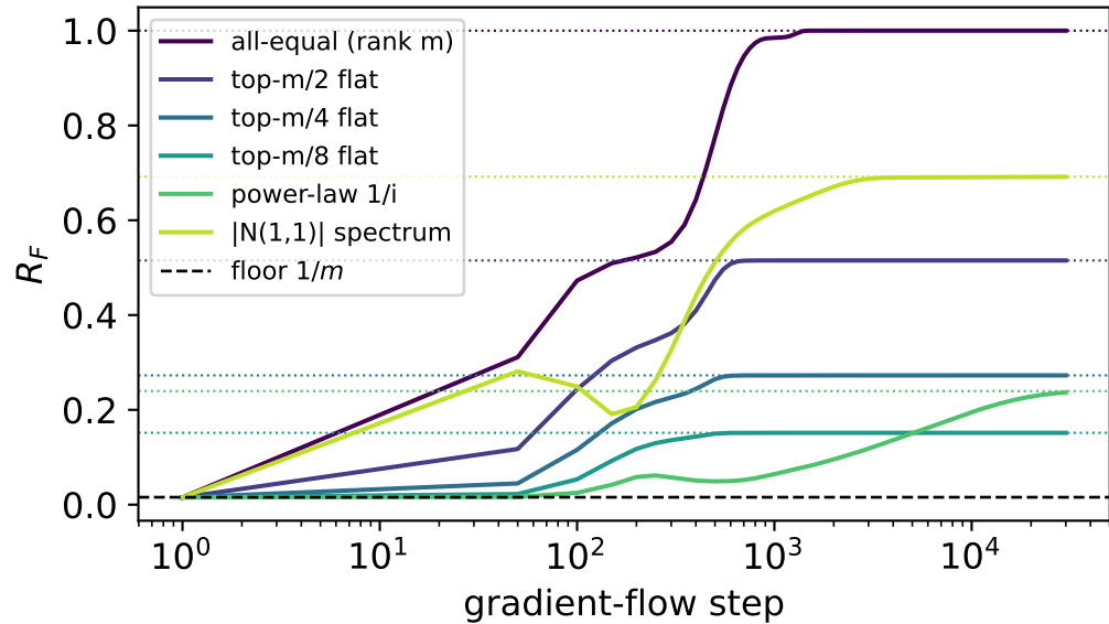
(a) Trajectory saturates at the predicted value
