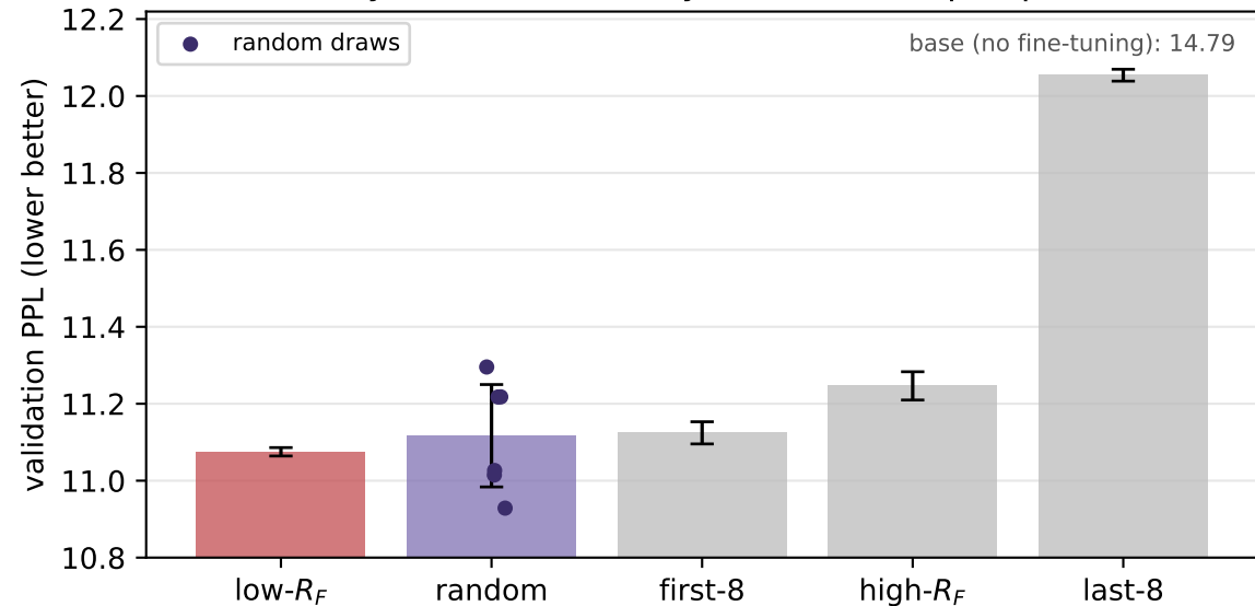
LoRA layer selection (8 layers, rank 8, equal params)
