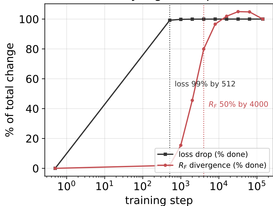
(c) Geometry lags loss ( \rho = 0.98 )
