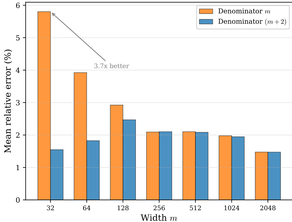
(b) Width convergence: m vs (m+2) denominator
