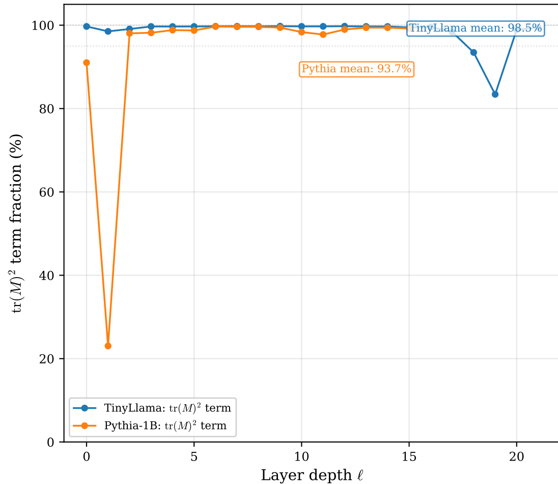
(b) Trace term dominance by layer
