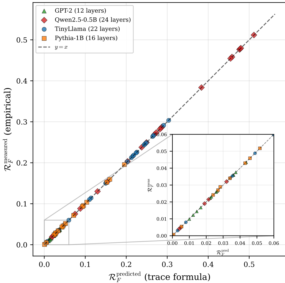
(a) Trace formula validation (74 layers, ratio 0.997-1.000)
