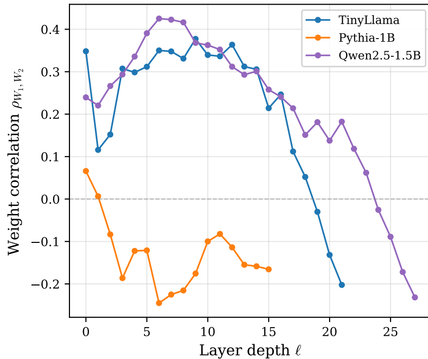
(b) Weight correlation vs depth
