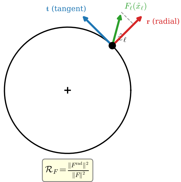
(a) Radial-tangential decomposition
