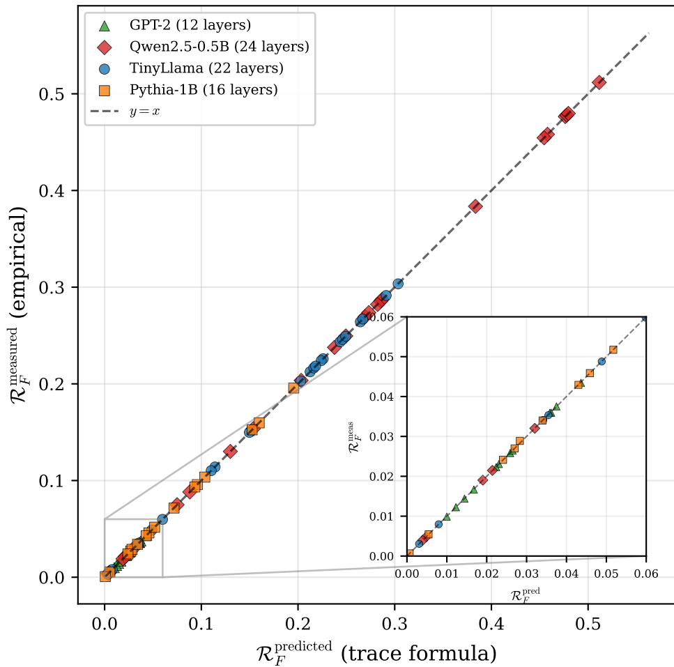
(a) Trace formula validation (74 layers, R^2=1.0000 )
