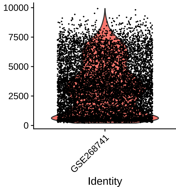
nFeature_RNA
