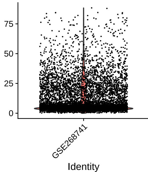
pct_mt
