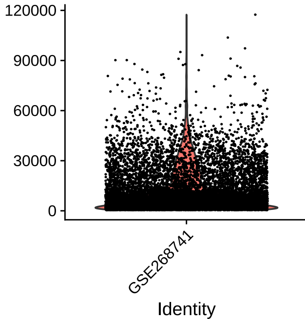
nCount_RNA
