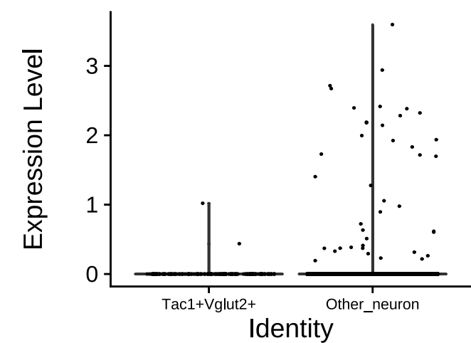
Klf2
