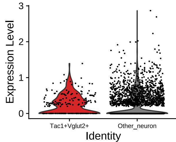
Slc17a6
