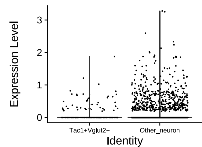
Tac1
