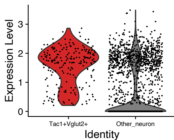
Slc17a6
