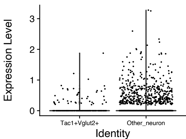
Tac1
