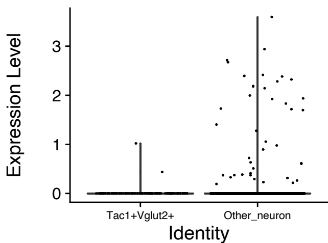
Klf2
