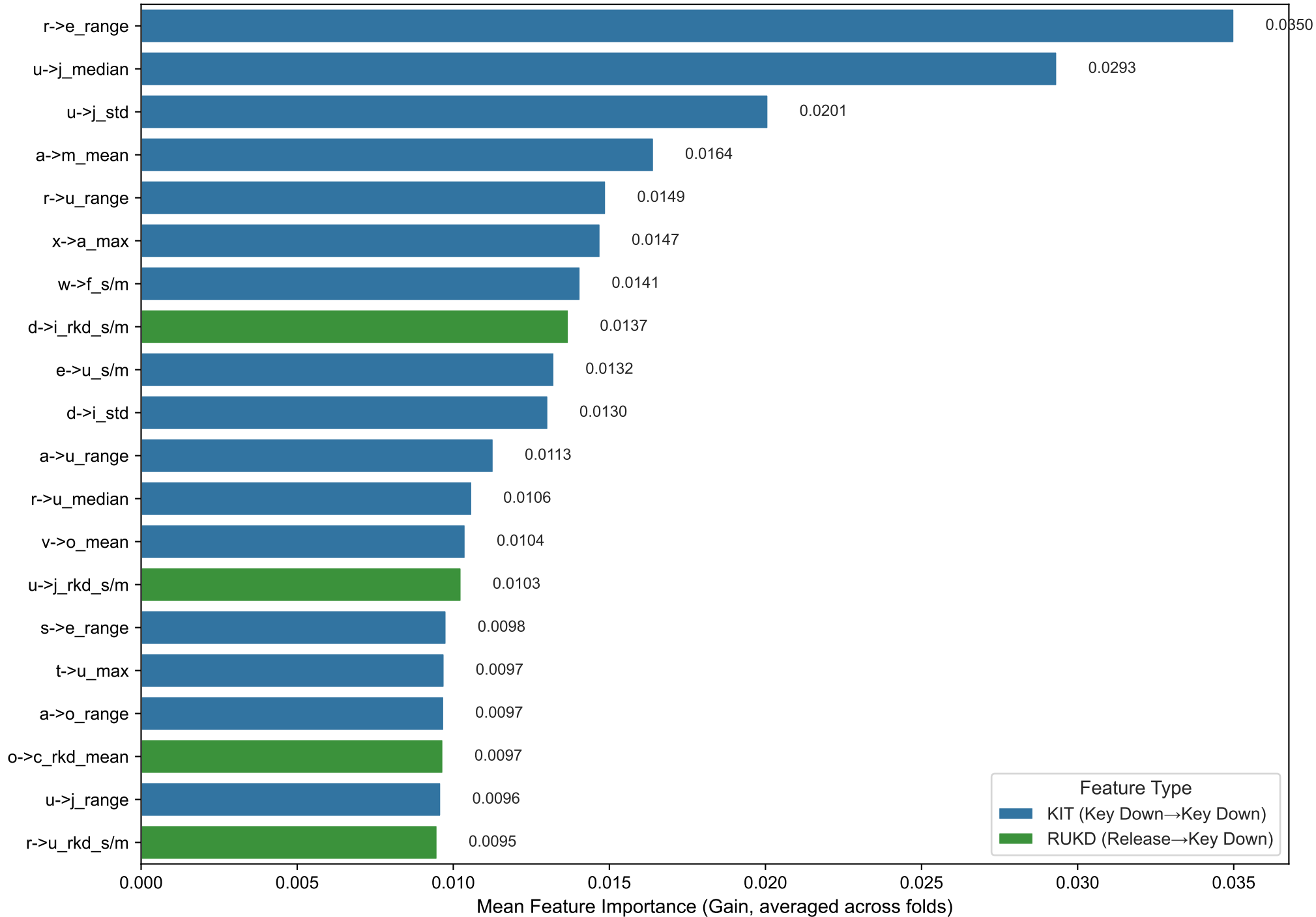
Top 20 Features — M2 (context-independent)
