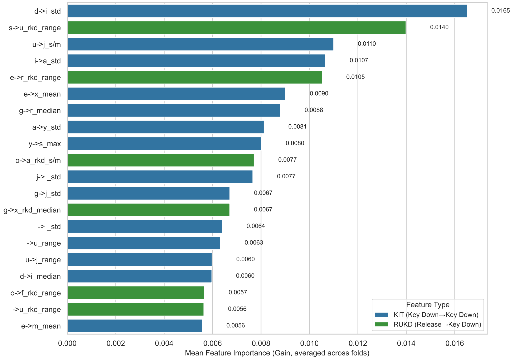
Top 20 Features — M3 (context-independent)
