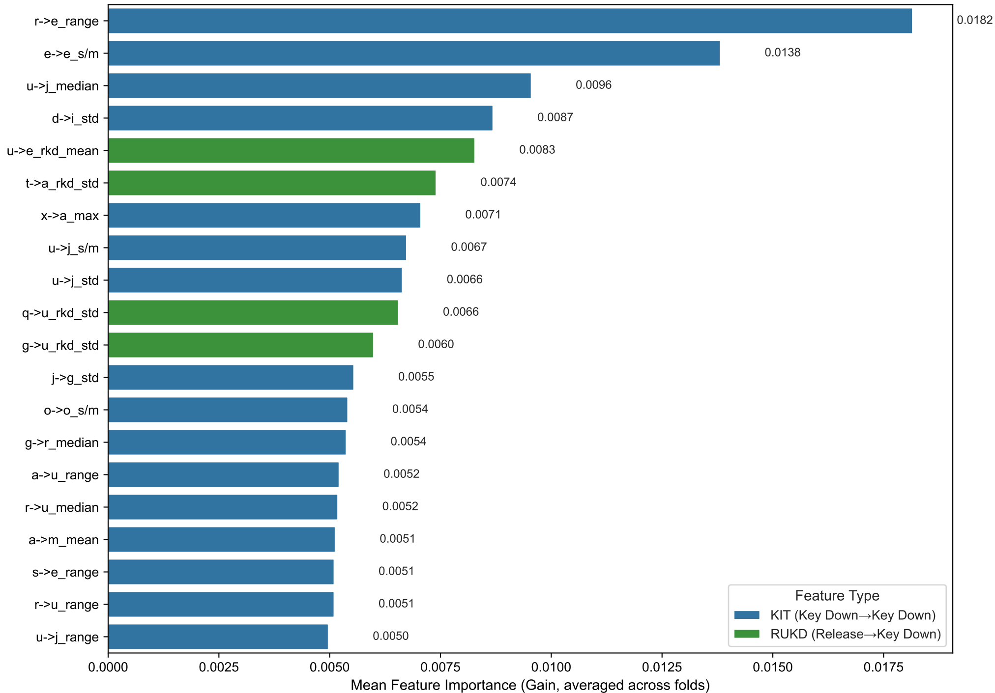
Top 20 Important Features
