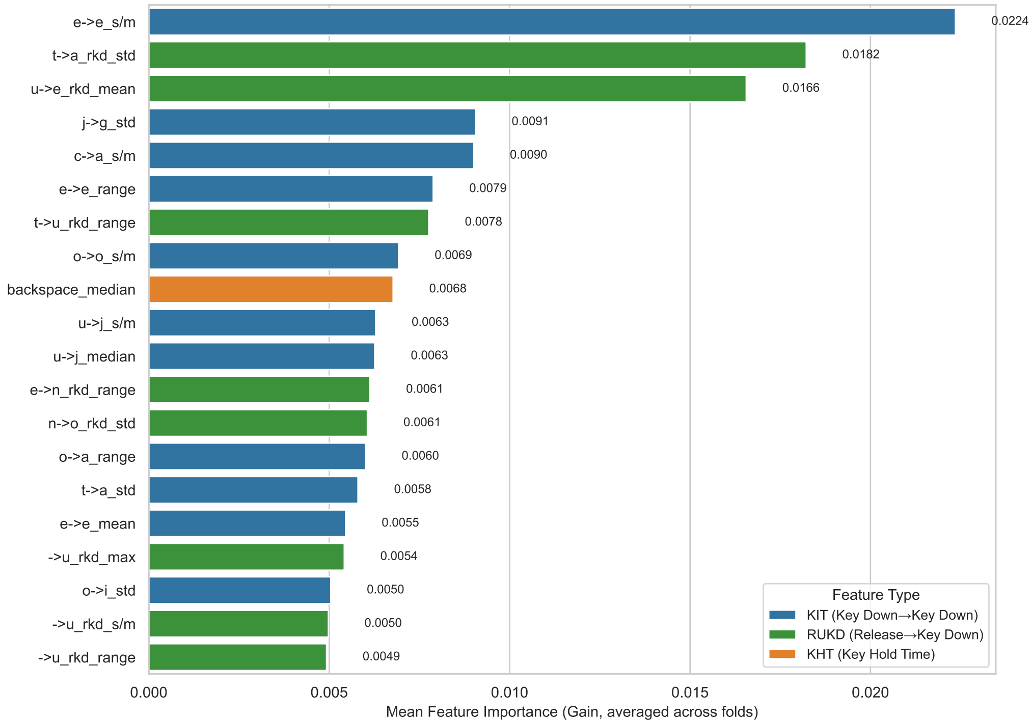
Top 20 Features — M5 (context-independent)
