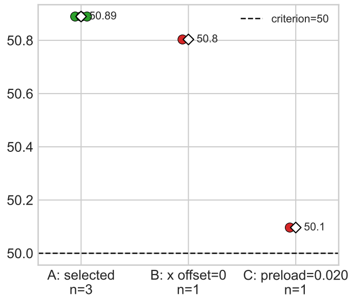
Object lift [mm]
