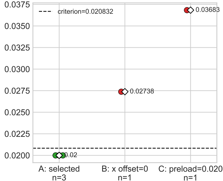
Peak hand-base acceleration [m/s 2 ]
