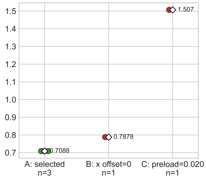
Relative slip [mm]
