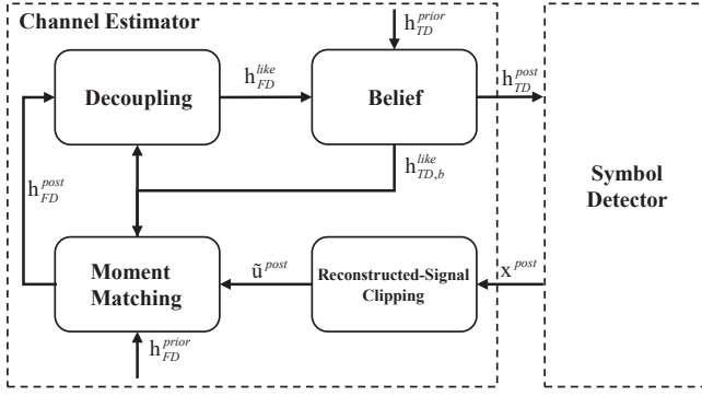
Fig. 3. The message flows of the CEP-based channel estimator.
