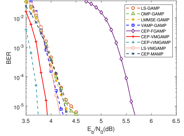
Fig. 15. BER performance of different joint channel estimation and symbol detection algorithms for QPSK OCDM LDPC-coded systems.
