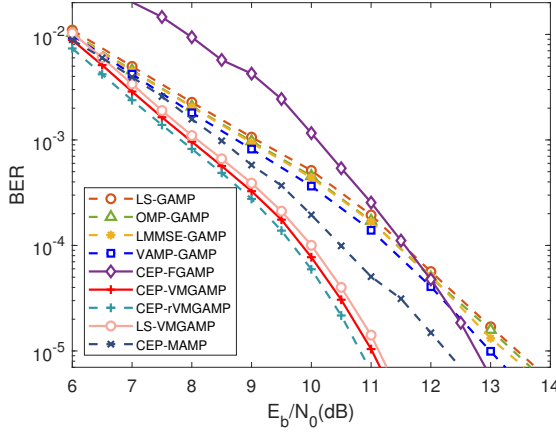
Fig. 13. BER performance of different joint channel estimation and symbol detection algorithms for QPSK OCDM uncoded systems.
