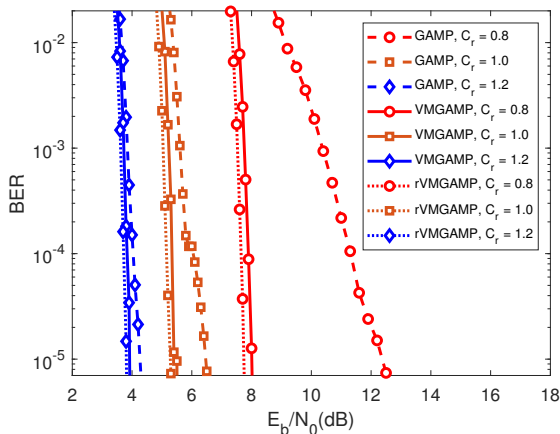
Fig. 10. BER performance for QPSK OCDM LDPC-coded systems with known CSI and different clipping thresholds.
