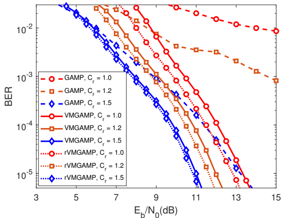
Fig. 9. BER performance for QPSK OCDM uncoded systems with known CSI and different clipping thresholds.
