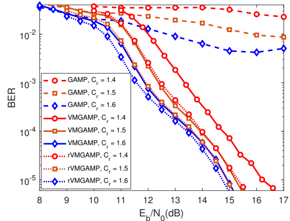
Fig. 11. BER performance for 16QAM OCDM uncoded systems with known CSI and different clipping thresholds.
