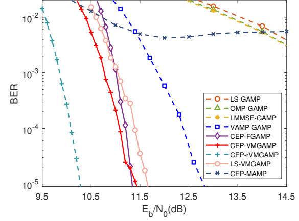
Fig. 16. BER performance of different joint channel estimation and symbol detection algorithms for 16QAM OCDM LDPC-coded systems.
