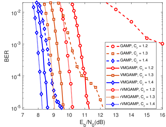
Fig. 12. BER performance for 16QAM OCDM LDPC-coded systems with known CSI and different clipping thresholds.
