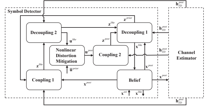
Fig. 4. The message flows of the VMGAMP-based symbol detector.
