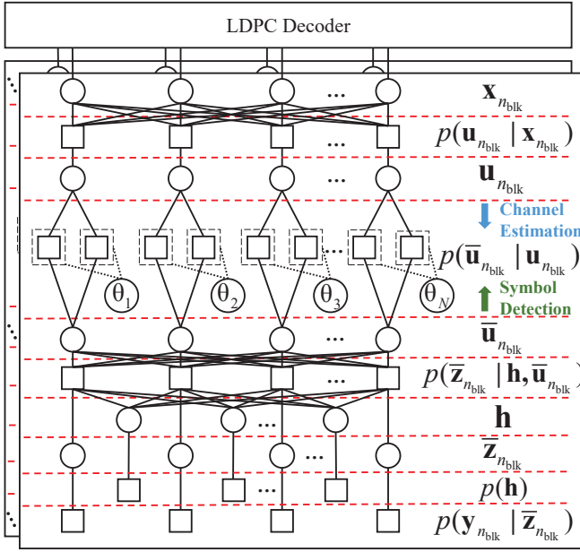
Fig. 2. Factor graph for joint channel estimation and symbol detection of OCDM signal with clipping distortion.
