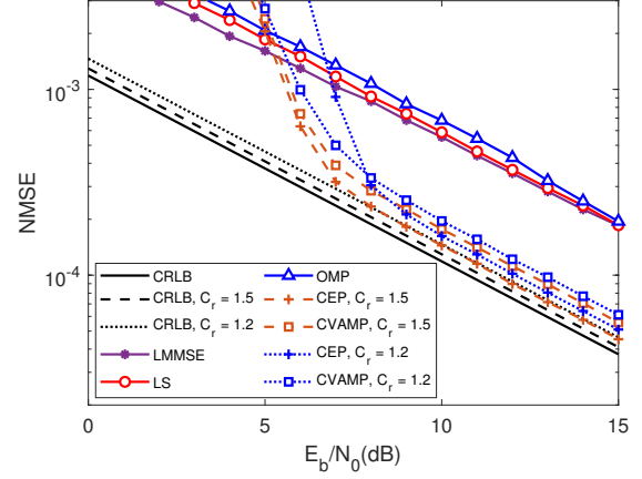
Fig. 7. NMSE performance of different channel estimation algorithms for QPSK OCDM uncoded systems.
