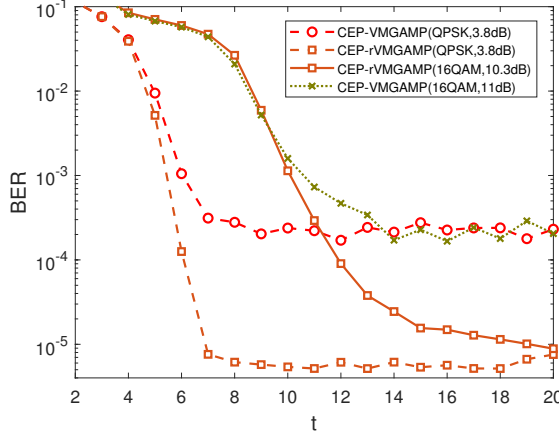
Fig. 5. BER performance of different algorithms with different numbers of turbo iterations for clipped OCDM LDPC-coded systems.
