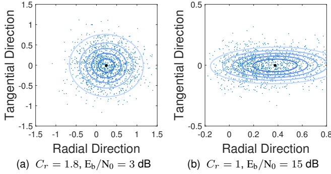
Fig. 6. Scatter plots of the phase-aligned effective-error samples. Each sample is rotated according to the corresponding phase used in the ICG update, so that the horizontal and vertical axes represent the radial and tangential components, respectively.
