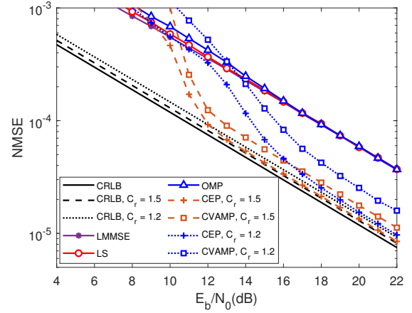
Fig. 8. NMSE performance of different channel estimation algorithms for 16QAM OCDM uncoded systems.
