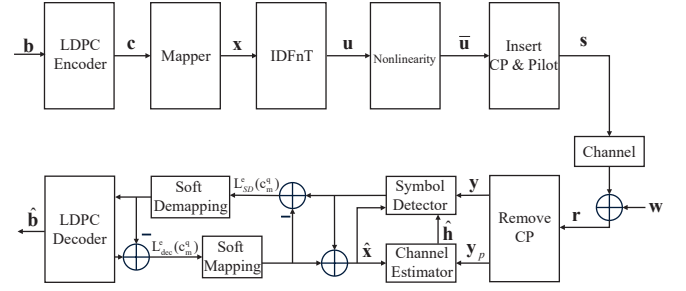
Fig. 1. The transceiver of the LDPC-coded OCDM system.
