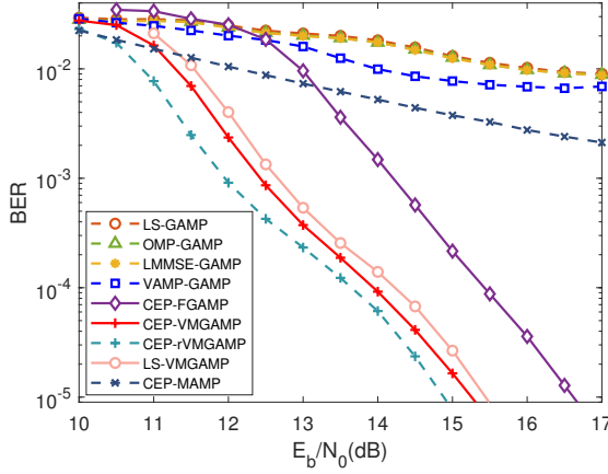
Fig. 14. BER performance of different joint channel estimation and symbol detection algorithms for 16QAM OCDM uncoded systems.
