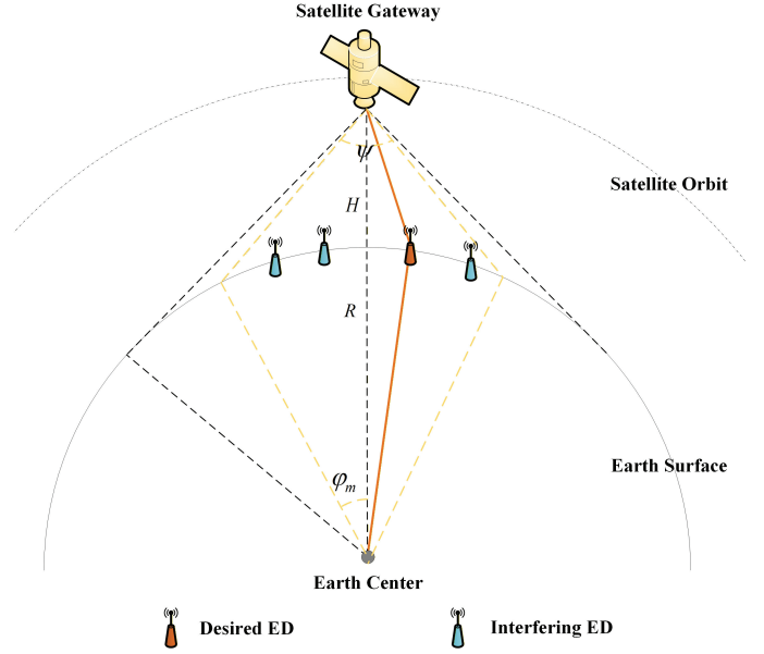
Fig. 1. Direct communications between the terrestrial LoRa EDs and the LEO satellite.
