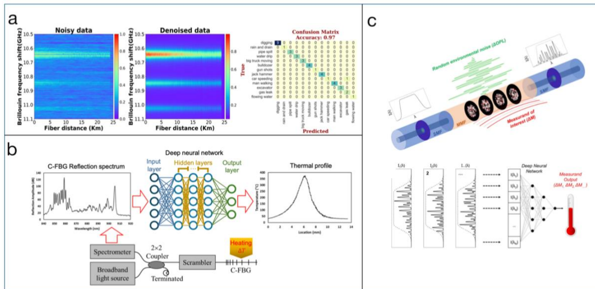
Figure 4. Learning-based denoising and robust demodulation in fiber sensors: (a) a deep-learning workflow denoises distributed Brillouin frequency-shift maps and classifies pipeline events (Adapted and reproduced with permission from Ref. [108]. Copyright 2024, Springer Nature); (b) a deep neural network maps chirped-FBG reflection spectra to subsurface thermal profiles during additive manufacturing (Adapted from Ref. [88]. Copyright 2024, Springer Nature; licensed under CC BY 4.0); and (c) a multimode-fiber interference sensor uses a deep neural network to recover the target measurand in the presence of strong optical-path-length noise (Adapted and reproduced with permission from Ref. [58]. Copyright 2021, Chinese Laser Press).
