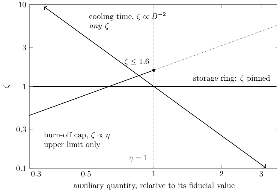
Figure 9. Why three observables with the same exponent give three different verdicts. Each locus is the set of parameter pairs consistent with one measurement; the horizontal axis is whatever must be known first and is not, namely nothing for the ring, \eta for the cap, B for a cooling time. All three scale as \zeta^{-1} and so respond equally; only the shape differs. The ring's locus is horizontal and fixes \zeta ; the cap's has slope one and is cut at \eta = 1 , which removes one side only, leaving an upper limit (the marked \zeta \leq 1.6 is for a 100 MeV cutoff); the cooling time's has slope -2 with no prior to cut it, so every \zeta survives. The exponent sets how strongly an observable responds; the geometry of its locus decides whether the response can be attributed to \zeta .
