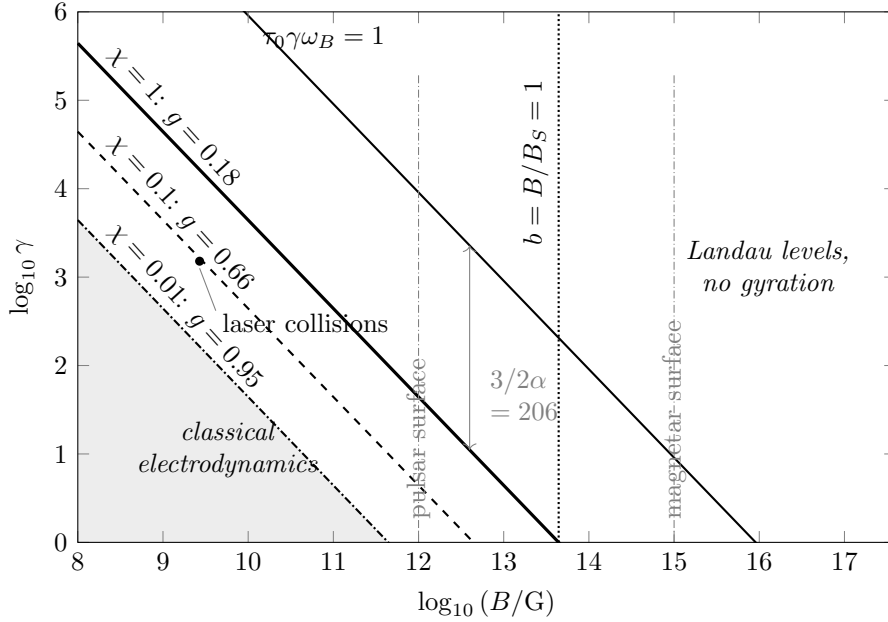
Figure 7. Where classical electrodynamics applies. Shaded is the region in which it is accurate to a few per cent: \chi \lesssim 0.01 and B \lesssim B_S . The three lines of constant \chi are labelled by the quantum suppression factor g of Eq. (107) that each carries, because the classical formula does not fail suddenly at any of them — it overstates the radiated power by 5% on the shaded boundary, by half at \chi = 0.1 , and by a factor of five at \chi = 1 . Crossing upward or to the right across any boundary leaves the classical domain, and the three kinds of boundary fail in different ways. Above \chi = 1 a single photon carries a sizeable part of the particle’s energy, so the emission is quantum and stochastic. To the right of B = B_S the transverse motion is Landau quantized and there is no gyration for an equation of motion to describe. The line \tau_0 \gamma \omega_B = 1 is where classical radiation reaction would itself become non-perturbative, which is the regime Secs. 1 to 5 are about — and it lies a factor 3/2\alpha = 206 above the line where the classical description of the emission has already failed, so it is never reached. Laser–electron collisions sit at \chi \approx 0.09 for a_0 = 10 at 800 nm against a \gamma = 1500 beam, the relevant field being the 2\gamma E seen head-on. That is a decade above the shaded region, not inside it: those experiments operate where the classical formula is already wrong by a third, which is why they can exclude it. Pulsar and magnetar surface fields are marked; at a magnetar surface even a mildly relativistic electron is already past both quantum boundaries.
