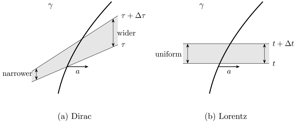
Figure 3. Where the 4/3 goes. Both panels show the same accelerating world line \gamma and the same slab of it, and differ only in what is being called “at the same moment”. (a) Dirac’s tube is built from the particle’s own succession of rest frames. Because the velocity changes along \gamma , successive slices are not parallel: they fan open on the side the particle is accelerating towards, and the slab is wider there. That fanning is the factor 1 + \varepsilon a \cdot n of Eq. (18). (b) Collecting field momentum at constant time in one chosen frame gives parallel slices and a slab of uniform thickness, with no such factor. The wedge by which the two shaded regions differ is worth exactly one third of the electromagnetic mass, which is the whole of the discrepancy between Eqs. (4) and (24).
