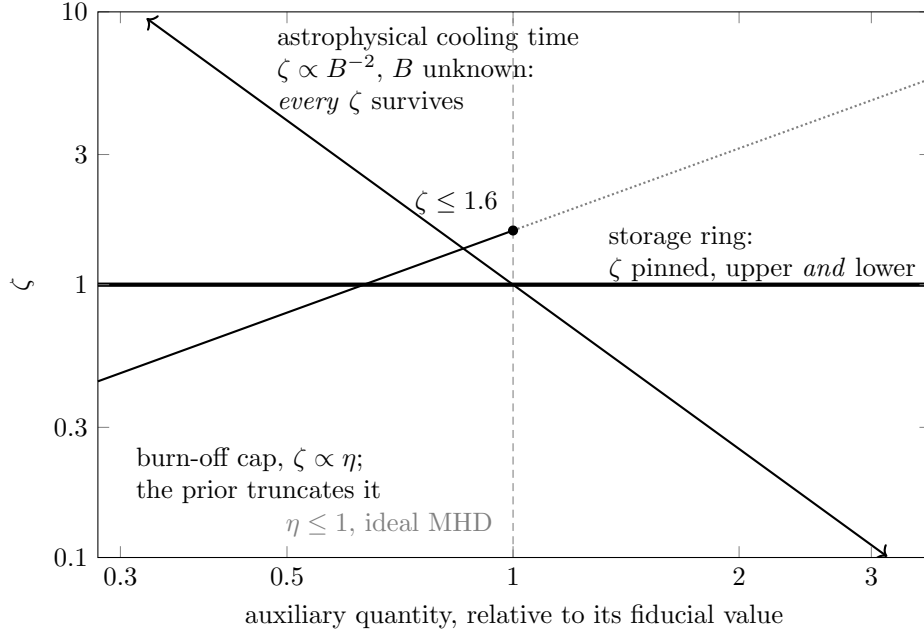
Figure 9. Why three quantities with the same exponent give three different verdicts. Each curve is the set of parameter pairs consistent with one measurement, in a plane whose horizontal axis is the quantity that has to be known before the measurement can be read and is not: nothing for the ring, \eta for the burn-off cap, B for an astrophysical cooling time. All three observables scale as \zeta^{-1} , so all three respond equally strongly to the coefficient; what differs is the shape of the locus and whether a prior cuts it. In a storage ring the auxiliary quantities are machine settings, the locus is horizontal, and \zeta is determined outright. The burn-off cap of Eq. (124) has cancelled B but not \eta , so its locus is a line of slope one; ideal magnetohydrodynamics caps \eta at unity, which truncates the line at the dashed vertical and leaves an upper limit on \zeta but no lower one. The value \zeta \leq 1.6 marked is what a source with a 100 MeV cutoff would give. An astrophysical cooling time retains B with no prior at all, its locus has slope -2 and runs off the frame in both directions, and every value of \zeta survives. The exponent sets how strongly the observable responds; the geometry of the locus decides whether the response can be attributed to \zeta rather than to something else.
