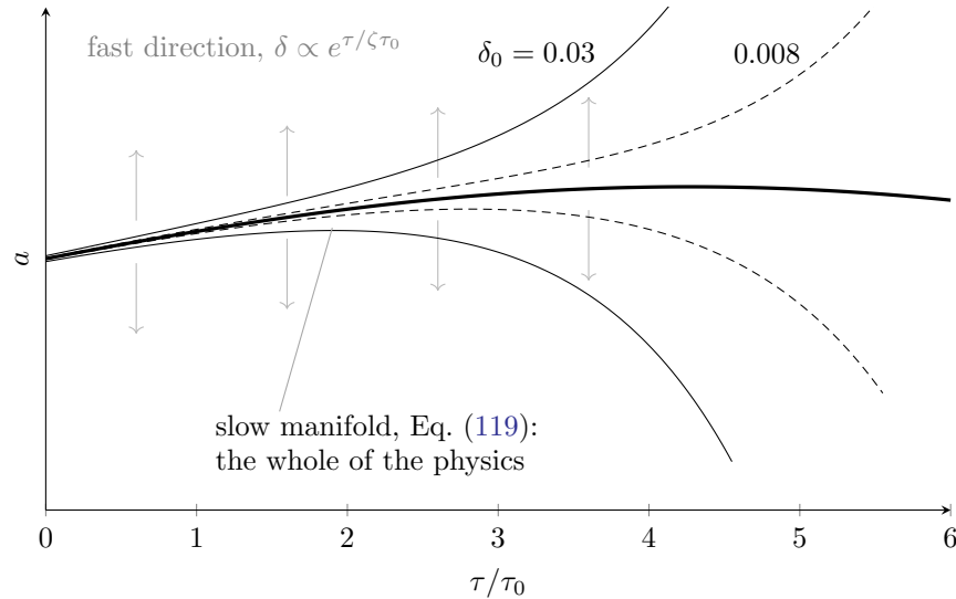
Figure 8. What reduction of order removes. The state space of the third-order equation (117) is (x, v, a) ; the heavy curve is the two-dimensional slow manifold on which a is fixed by the applied force through Eq. (96), and the vertical arrows are the remaining direction, along which perturbations grow as e^{\tau/\zeta\tau_0} . Four trajectories are shown starting off the manifold by \delta_0 = \pm 0.03 and \pm 0.008 in units of the force; they leave the frame after \ln(1/\delta_0) times \zeta\tau_0 , and no choice of \delta_0 avoids this, only postpones it logarithmically. Reduction of order is the restriction to the heavy curve, and Eq. (119) is its equation. The figure also shows why the removed object is a coordinate of the state space and not a coefficient: \zeta sets the rate at which the thin curves depart, and moving it slides the arrows without moving the heavy curve at all.
