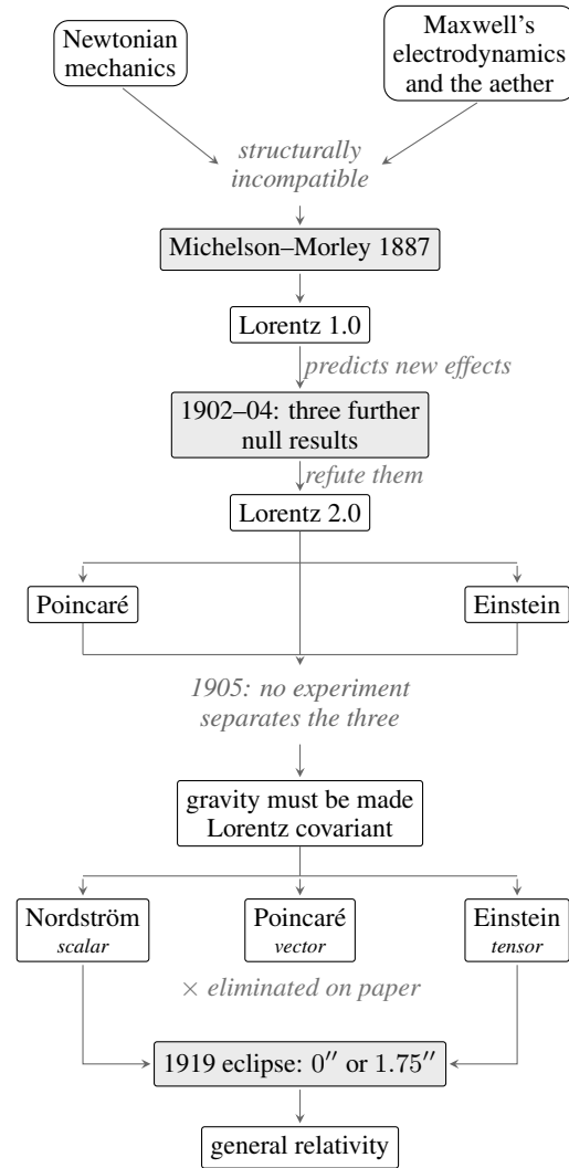
Figure 1. The theory space, from the two sources to general relativity, with shaded boxes marking the points at which the world had to answer. The vector theory falls on paper, the scalar only in 1919.
