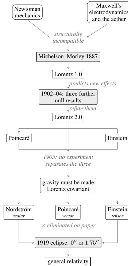
Figure 1. The theory space from classical physics to general relativity, with shaded boxes as the key experiments.
