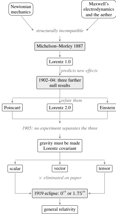
Figure 1. The theory space, from the two sources to general relativity. Shaded boxes are the points at which the world had to answer, the same convention used in Tables 1 and 2. The vector theory is eliminated before any observable is computed. The scalar theory survives every calculation and is eliminated only in 1919.
