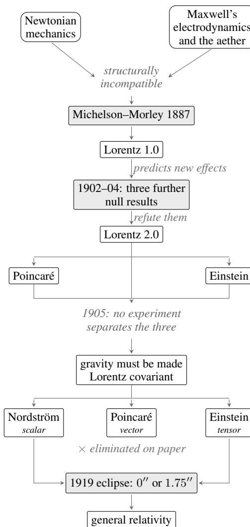
Figure 1. The theory space, from the two sources to general relativity. Shaded boxes are the points at which the world had to answer, the same convention used in Tables 1 and 2. The vector theory is eliminated before any observable is computed. The scalar theory survives every calculation and is eliminated only in 1919.
