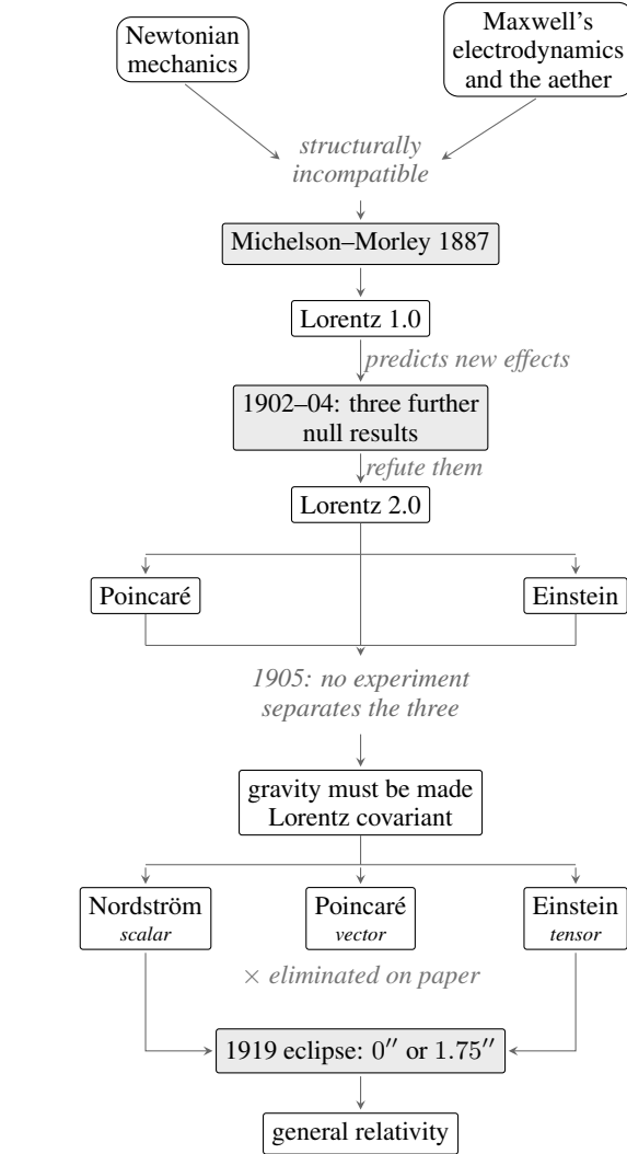
Figure 1. The theory space from classical physics to general relativity, with shaded boxes as the key experiments.
