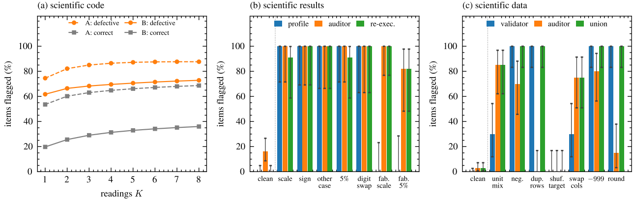
Figure 2. What each tier flags. (a) Scientific code: the shipped auditor’s union flag rate against the number of readings, on defective (orange) and correct (grey) instances, in arm A, whose task gave the whole problem (dashed), and arm B, whose task was reframed around the step (solid). (b) Scientific results and (c) scientific data, by fault type, with clean items leftmost: the deterministic tier (blue: the science profile in b, the card-derived validator in c), the LLM auditor at four readings (orange), and re-execution (b) or the union of the two (c) in green. The LLM’s flag is any model BLOCKER in the union of readings; the profile’s is a hard failure, the validator’s any fired check, re-execution’s a value outside np.allclose defaults. Bars carry exact binomial 95% intervals on the item counts (supplementary; they ignore clustering).
