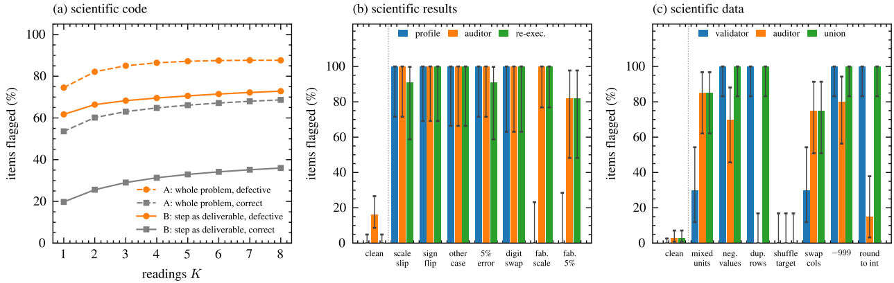
Figure 2. What each tier flags. (a) Scientific code: the shipped auditor’s union flag rate against the number of readings, on defective (orange) and correct (grey) instances, in the registered arm that gave the whole problem as the task (dashed) and the arm that named the step as the deliverable (solid). (b) Scientific results and (c) scientific data, by fault type, with clean items leftmost: the deterministic tier (blue: the science profile in b, the card-derived validator in c), the LLM auditor at four readings (orange), and re-execution (b) or the union of the two (c) in green. Bars carry exact binomial 95% intervals on the item counts (supplementary; they ignore clustering). Registered flag rule throughout: any model BLOCKER in the union of readings.
