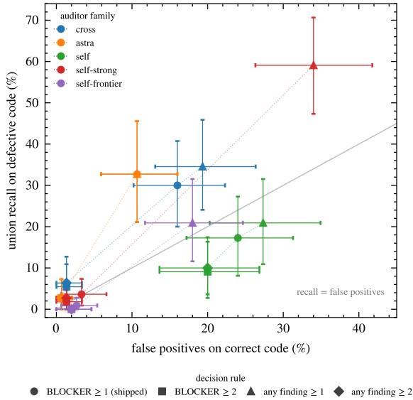
Figure 2. Flag coverage is a property of the decision rule, not only of the auditor. Each point is one auditor family re-graded under one of four decision rules on the same archived readings, with problem-cluster 95% intervals on both axes; no new model calls were made. The dotted guides join a family’s four points and are not a measured curve — only the four points exist. Two things the accompanying table cannot show: the families do not lie on one frontier, and self-strong has no reachable point between 3.3% and 34.0% false positives, which is exactly where a comparison matched to the cross-vendor auditor would sit, so its ranking there is bracketed rather than measured. Nothing in this figure assesses finding content ; a flag is not a diagnosis.
