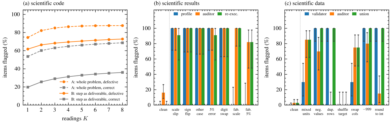
Figure 4. What each tier flags. (a) Scientific code: the shipped auditor’s union flag rate against the number of readings, on defective (orange) and correct (grey) instances, in the registered arm that gave the whole problem as the task (dashed) and the arm that named the step as the deliverable (solid). (b) Scientific results and (c) scientific data, by fault type, with clean items leftmost: the deterministic tier (blue: the science profile in b, the card-derived validator in c), the LLM auditor at four readings (orange), and re-execution (b) or the union of the two (c) in green. Bars carry exact binomial 95% intervals on the item counts (supplementary; they ignore clustering). Registered flag rule throughout: any model BLOCKER in the union of readings.
